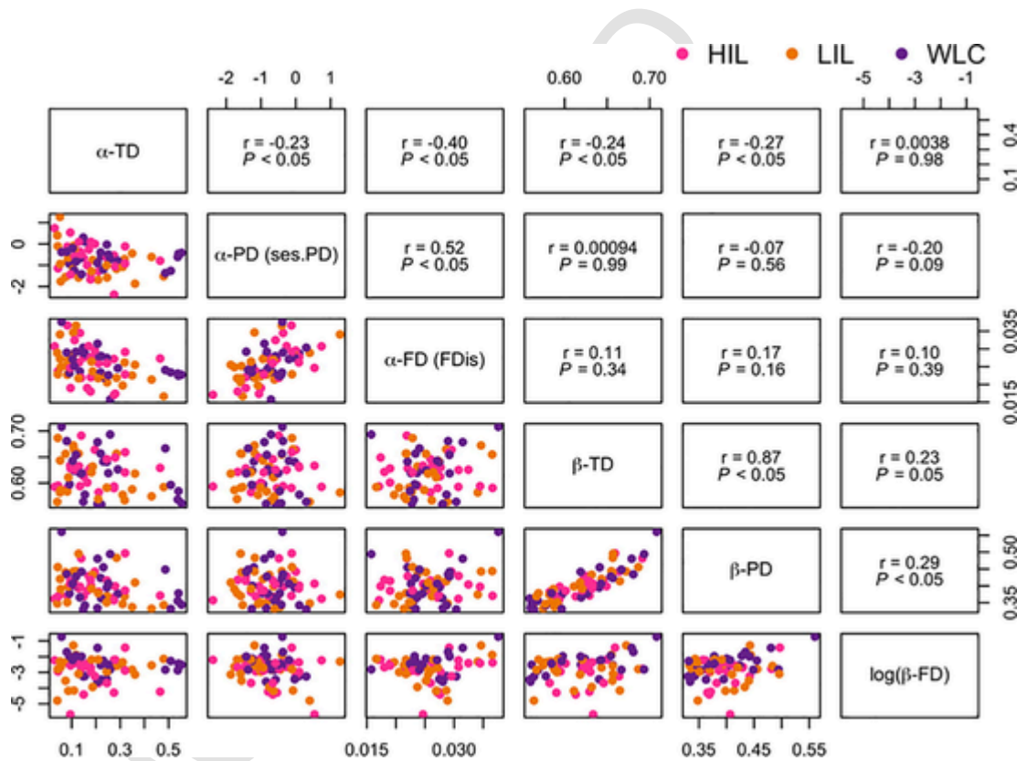
Fig. 6. Pearson correlations between all diversity metrics: \alpha - and \beta -taxonomic (TD), phylogenetic (PD), and functional (FD) in yards (HIL = high-input lawns; LIL = low-input lawns; WLC = wildlife-certified yards). Alpha-taxonomic diversity was calculated as species richness normalized by plot area. Alpha-phylogenetic and functional diversity were calculated as the standardized effect size of Faith's PD (ses.PD) and Functional Dispersion (FDIs), respectively. Beta-diversity for each site was calculated as the site distance to its group centroid.
