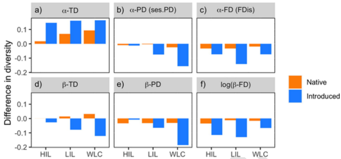
Fig. 5. Differences in the variance of \alpha -diversity (measured as standard deviation) and mean \beta -diversity of each biodiversity component (i.e., taxonomic [TD], phylogenetic [PD], and functional [FD]) associated with native and introduced species across yard types. Differences associated with each pool of species were calculated as the diversity value including both natives and introduced species, minus the diversity value without that pool of species. Diversity values were previously standardized to allow comparisons. Negative values indicate the pool of species contributed to homogenization, while positive values indicate the pool of species contributed to differentiation. HIL = high-input lawns; LIL = low-input lawns; WLC = wildlife certified yards.
